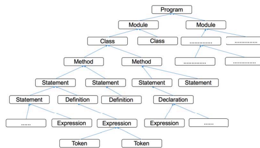
Figure 1: Abstract syntax trees – illustration of code hierarchical structure and composability.
